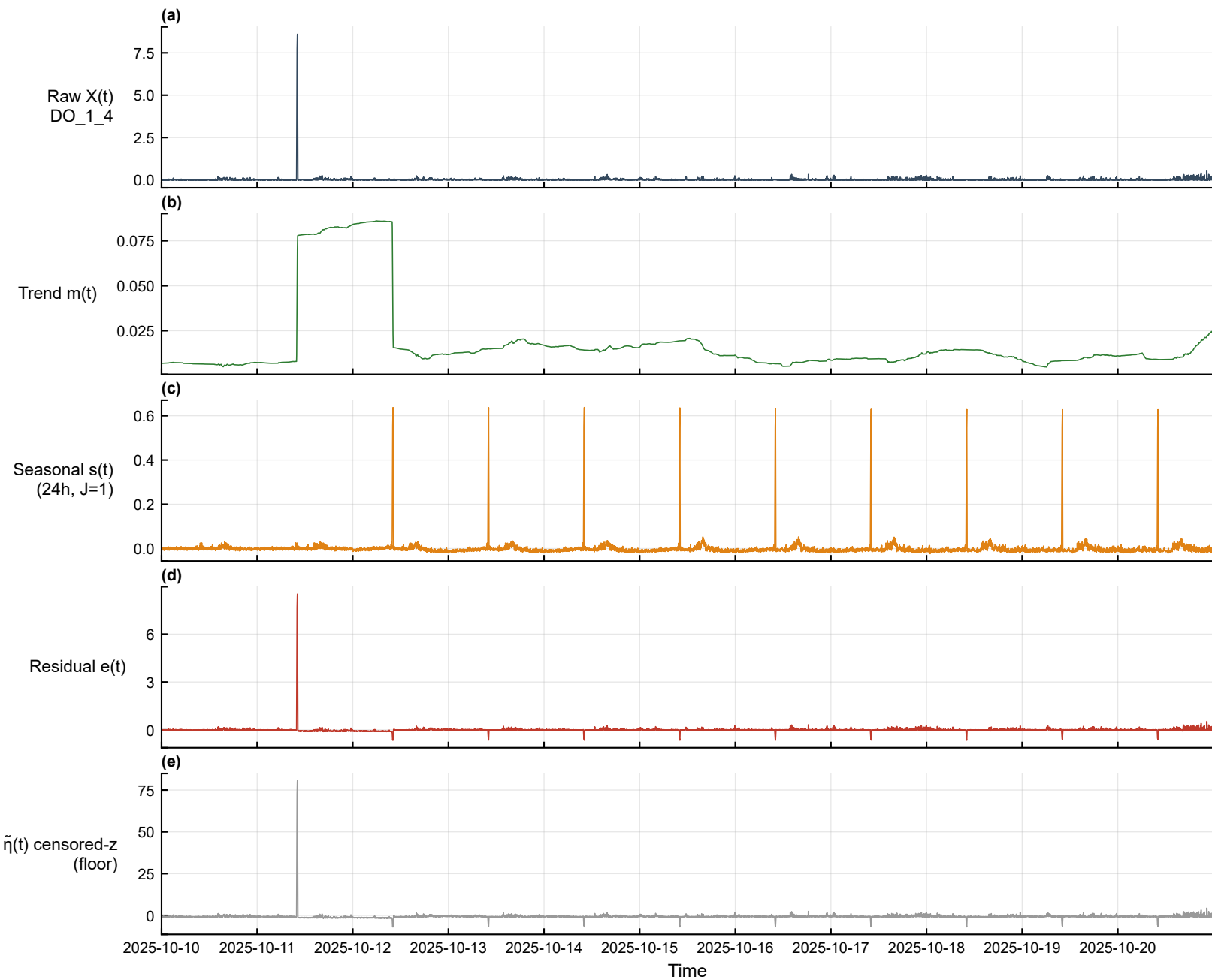
Multi-scale decomposition — DO_1_4 (post_anoxic, min) [2025-10-10~2025-10-20]
